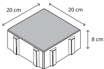
Joint 7 mm
